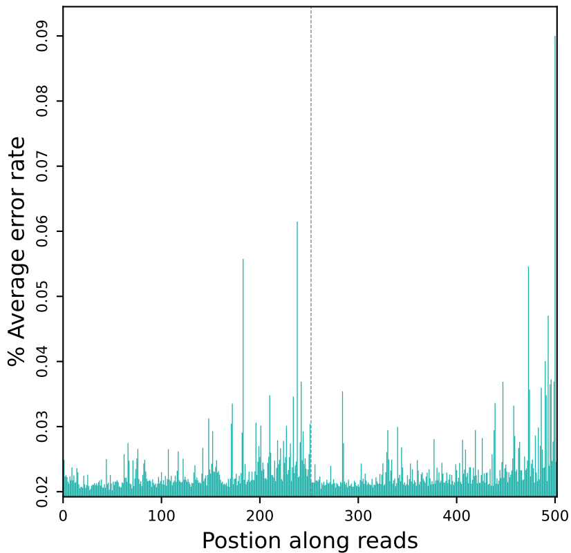
Error rate distribution along reads (R20111)
